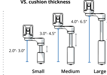
Hardware size VS. cushion thickness
